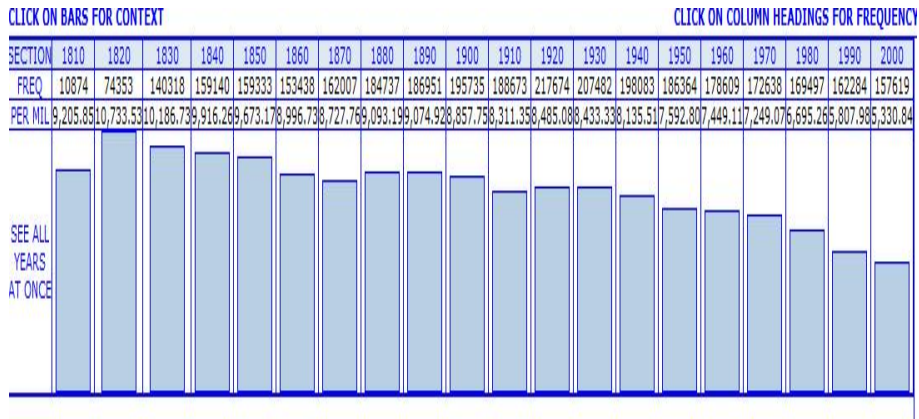
Figure 3: Frequency of the be -passive in the COHA
