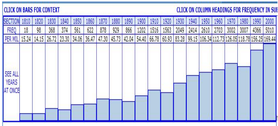
Figure 2: Frequency of the get -passive in the COHA
